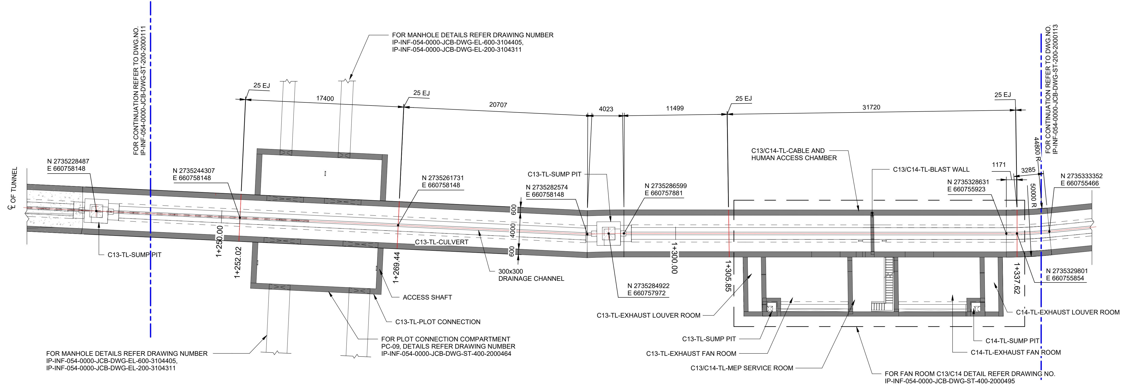
1 C-13/C-14 MV CULVERT ROAD LEVEL PLAN 1 : 200
