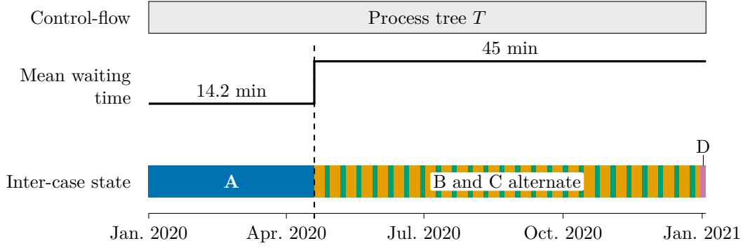
Figure 1.1: Visualisation of the synthetic Rheon log generated with mean waiting time drift. At the drift point (dashed), the mean waiting time between consecutive events of a case rises from 14.2 to 45 min, while all cases still follow process tree T . The inter-case state of each 12-hour window switches exactly there from A to an alternation of B and C, D marks the run-out of the log after the last case arrivals.
