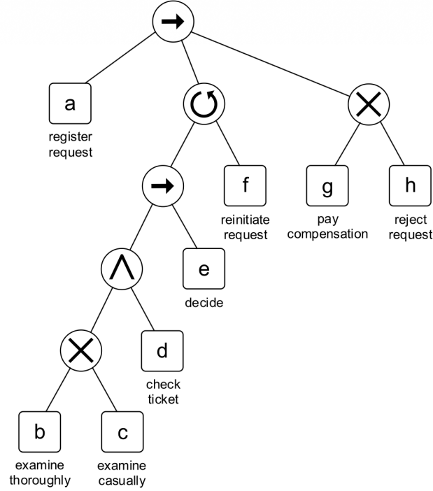
Figure 3.1: The process tree \rightarrow(a, \odot(\rightarrow(\wedge(\times(b, c), d), e), f), \times(g, h)) showing different process tree operators. Taken from van der Aalst [25].
