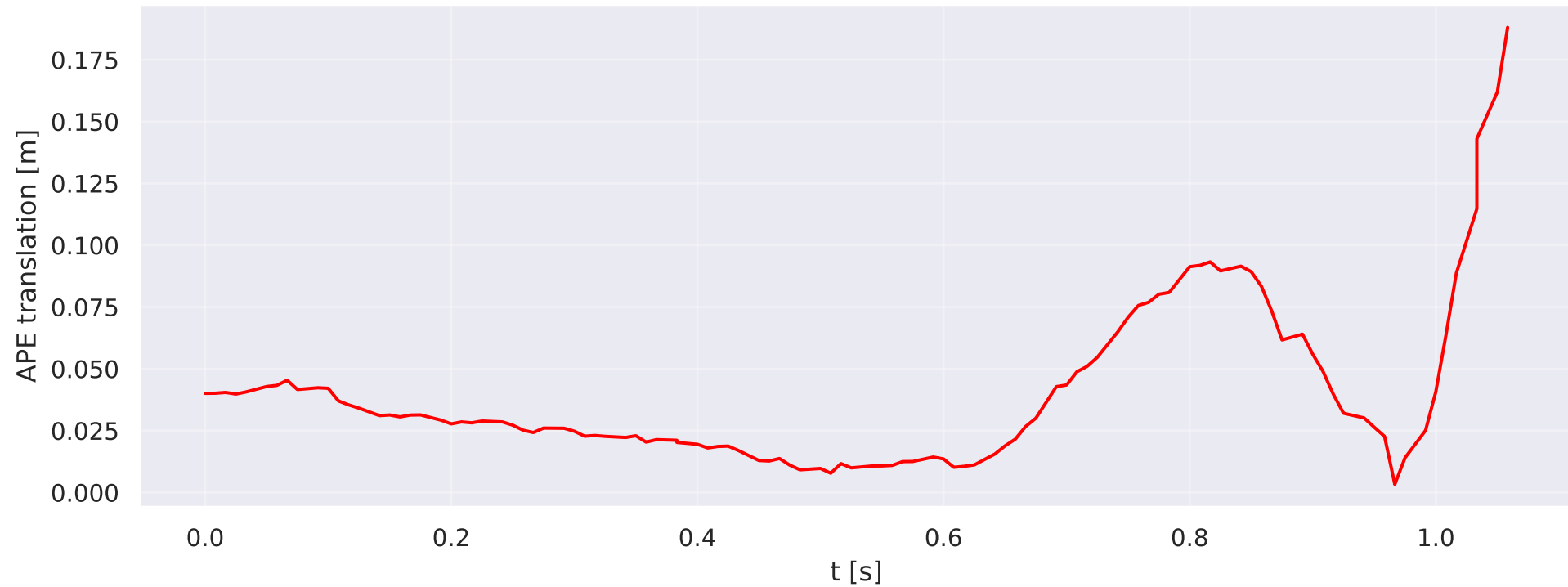
esvo2/vector/mountain-fast — APE over time
