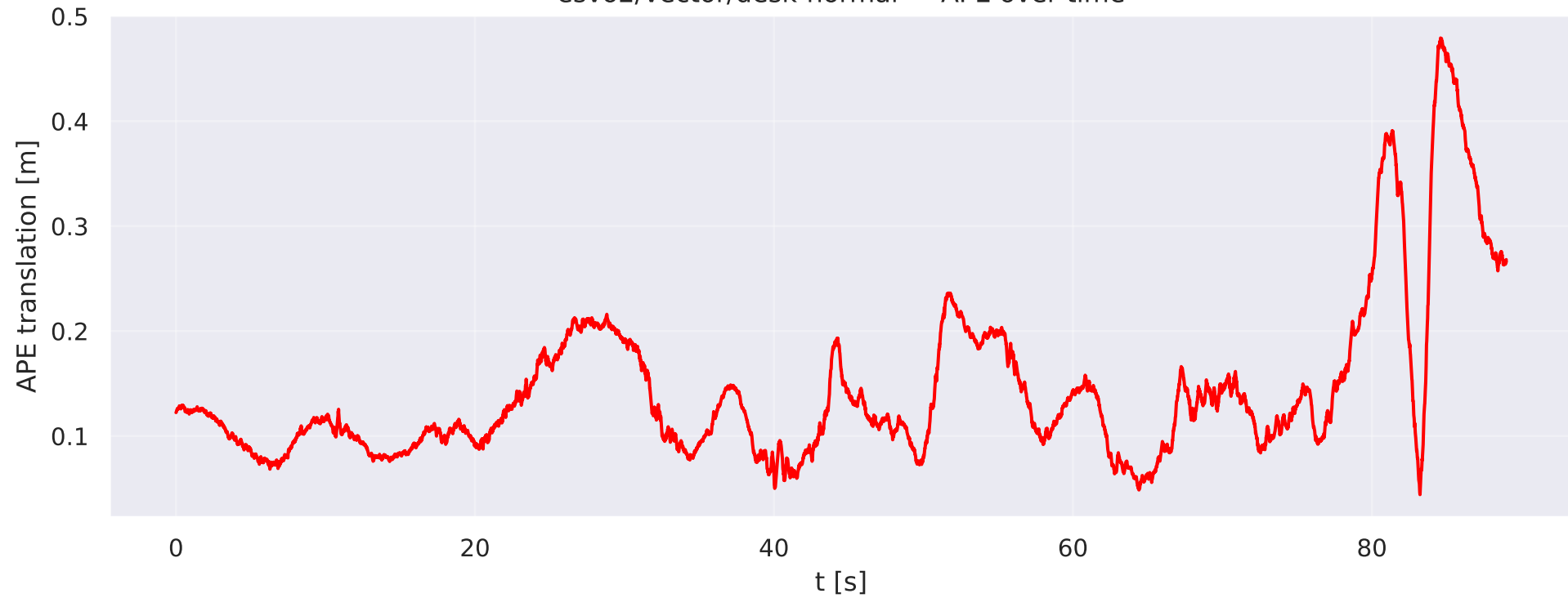
esvo2/vector/desk-normal — APE over time
