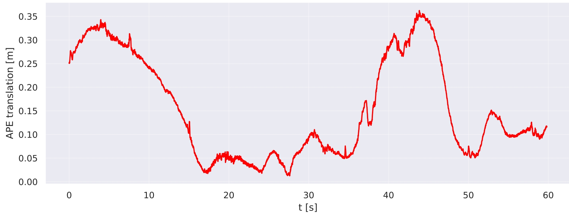
esvo2/vector/hdr-normal — APE over time
