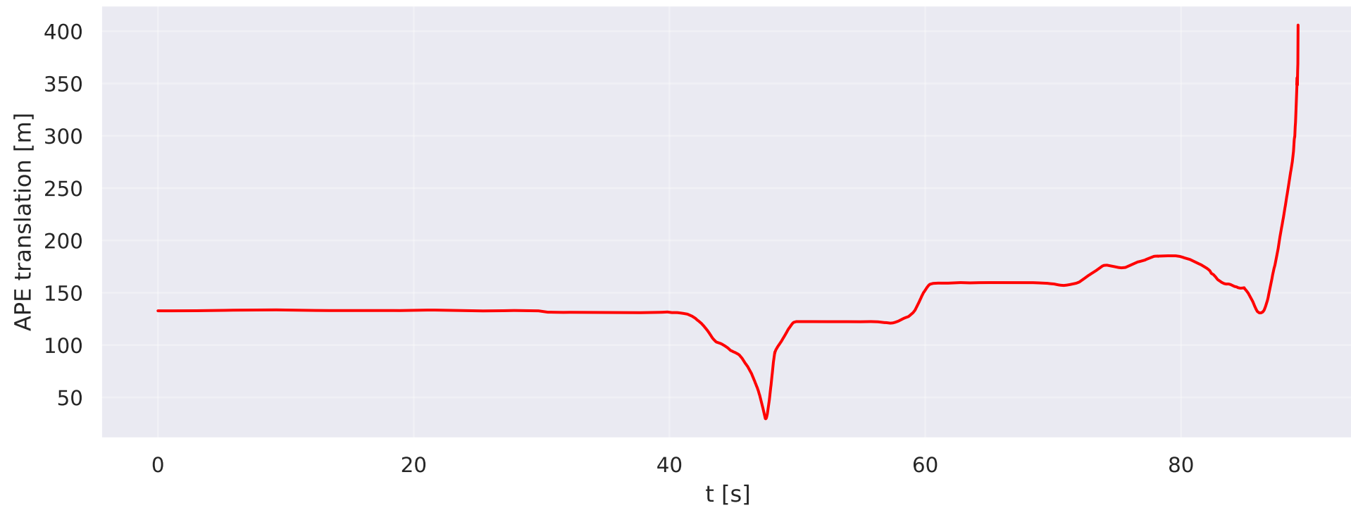
esvo2/vector/sofa-normal — APE over time
