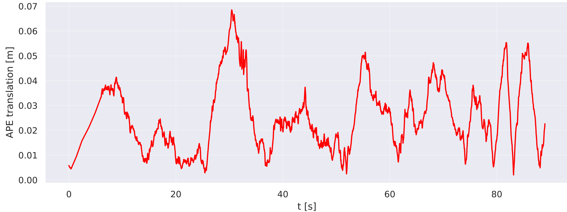
deio/vector/desk-normal (Sim3) — APE over time
