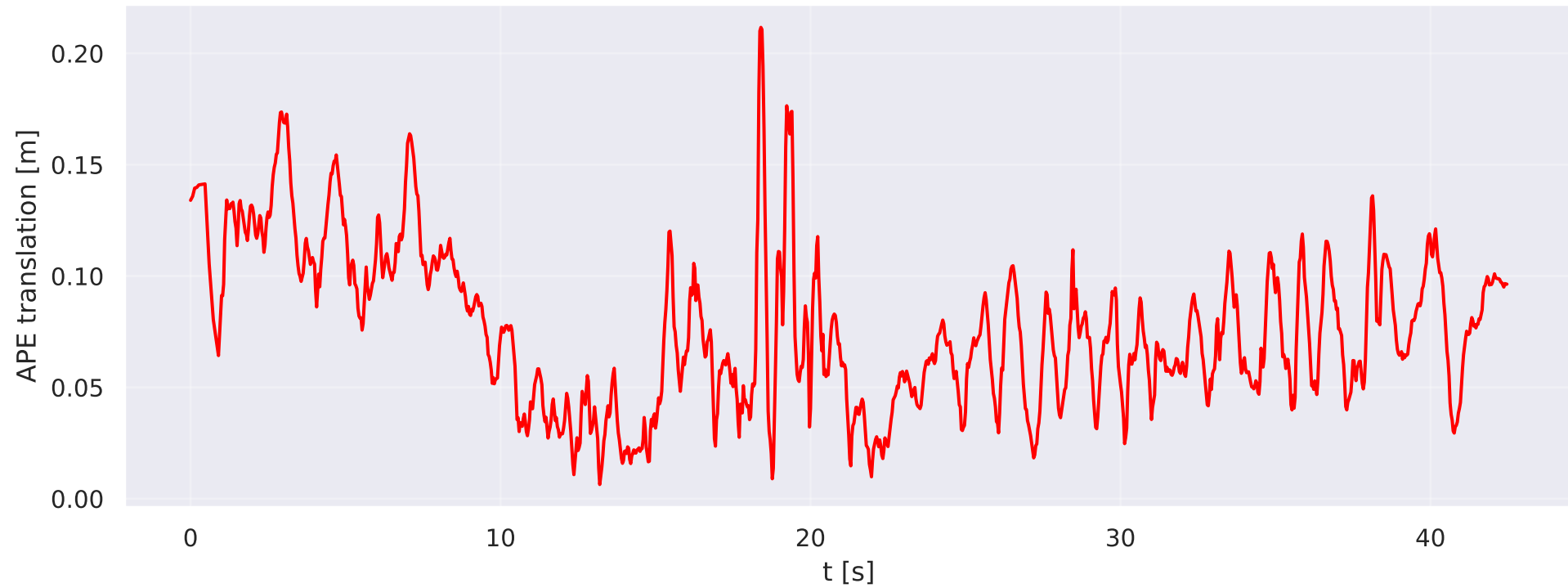
deio/vector/mountain-fast (Sim3) — APE over time
