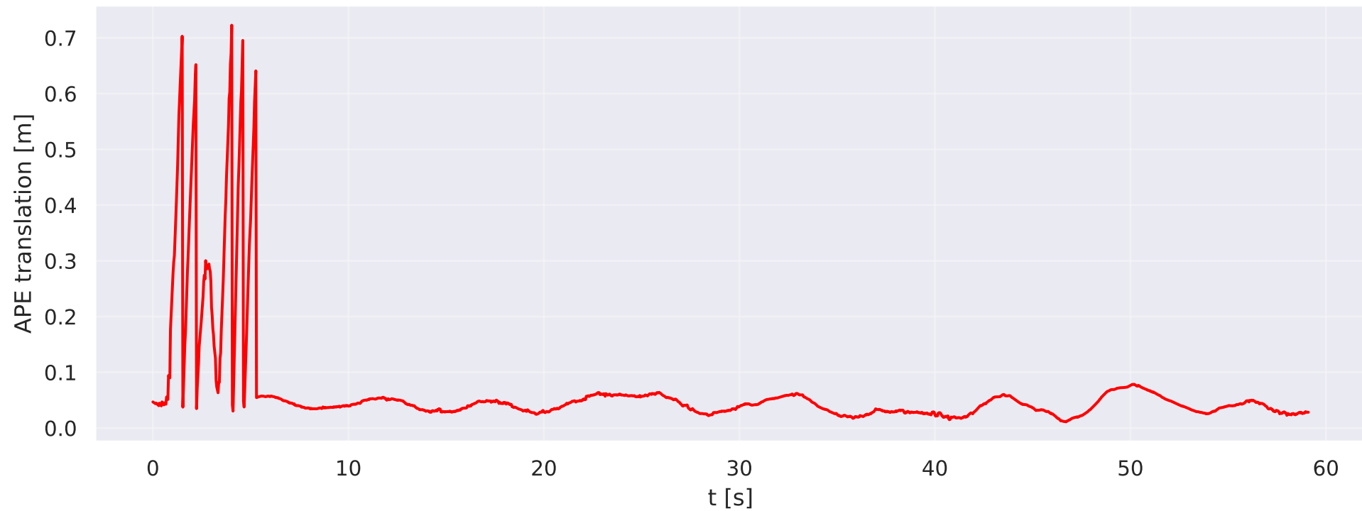
deio/vector/mountain-normal (Sim3) — APE over time
