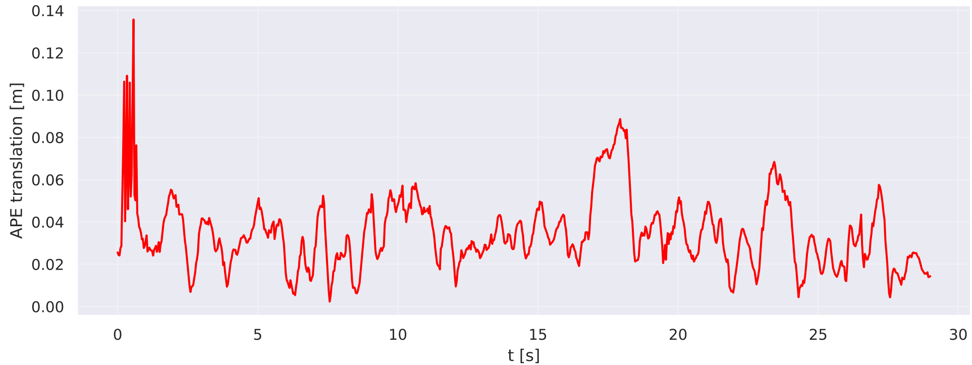
deio/vector/robot-fast (Sim3) — APE over time
