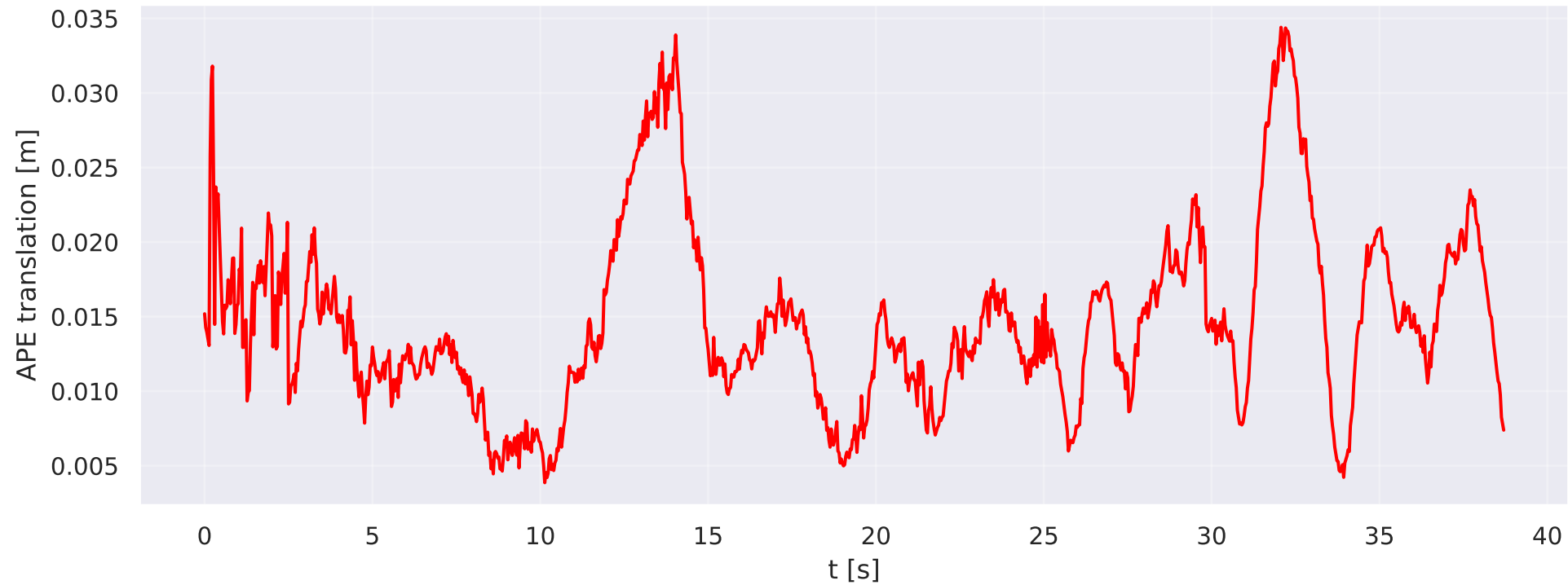
deio/vector/robot-normal (Sim3) — APE over time
