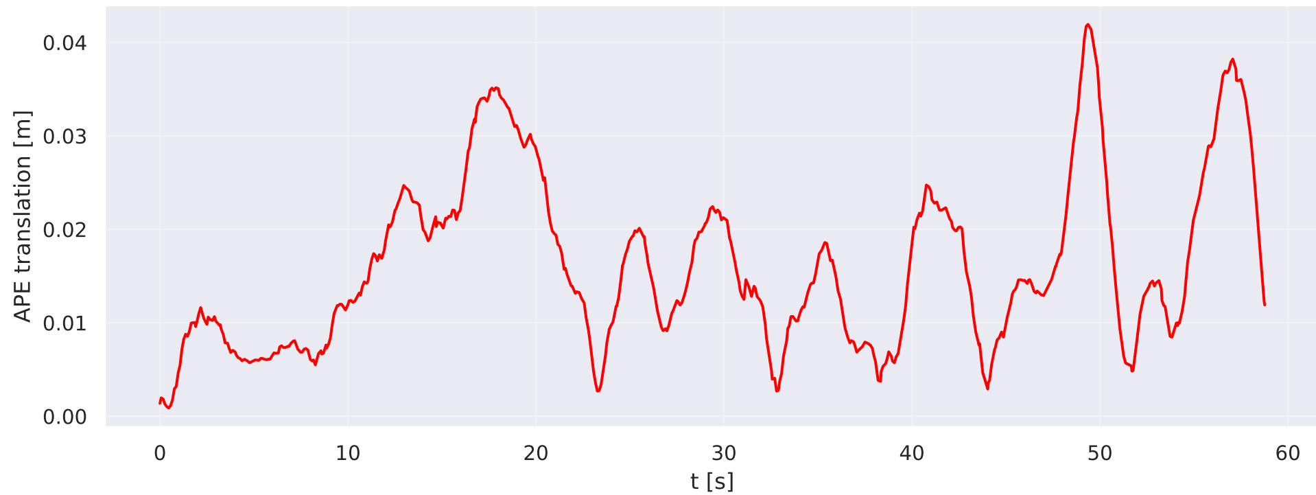
esvio/vector/hdr-normal — APE over time
