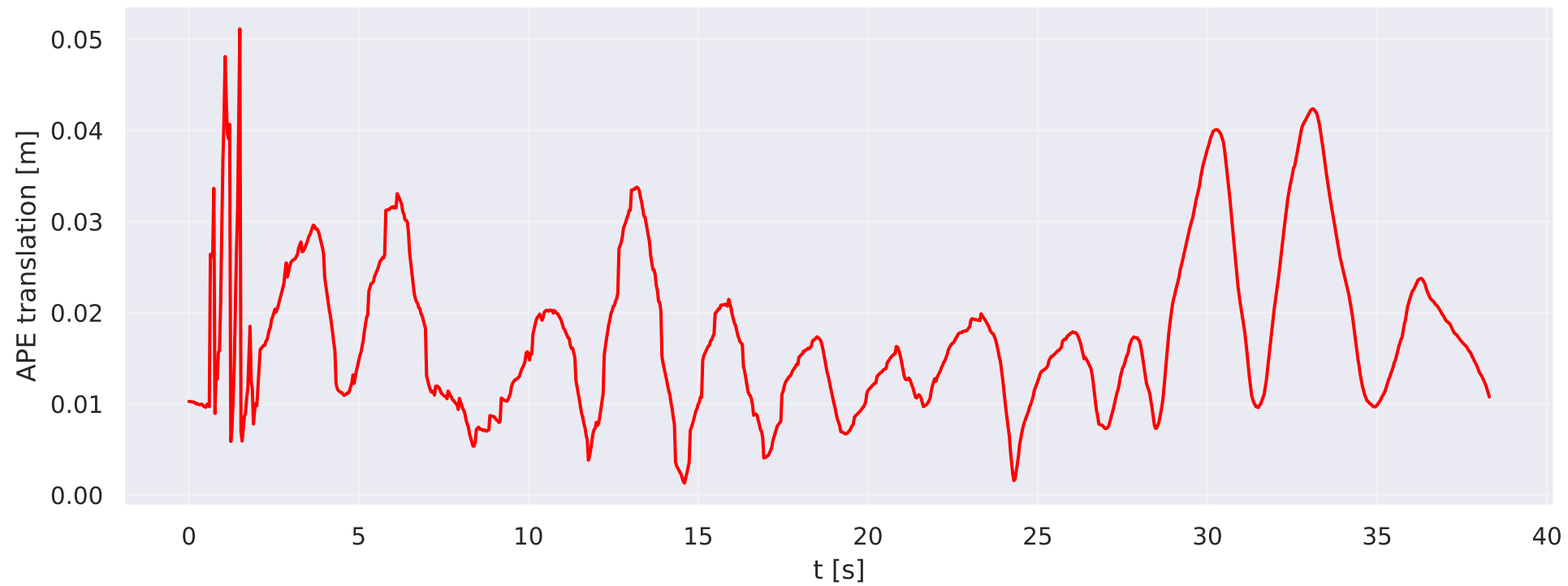
corner-slow DEIO(our run) — APE over time
