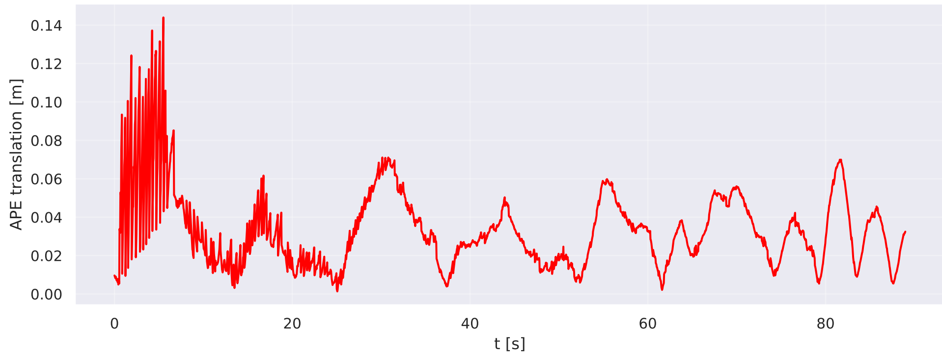
desk-normal DEIO(our run) — APE over time
