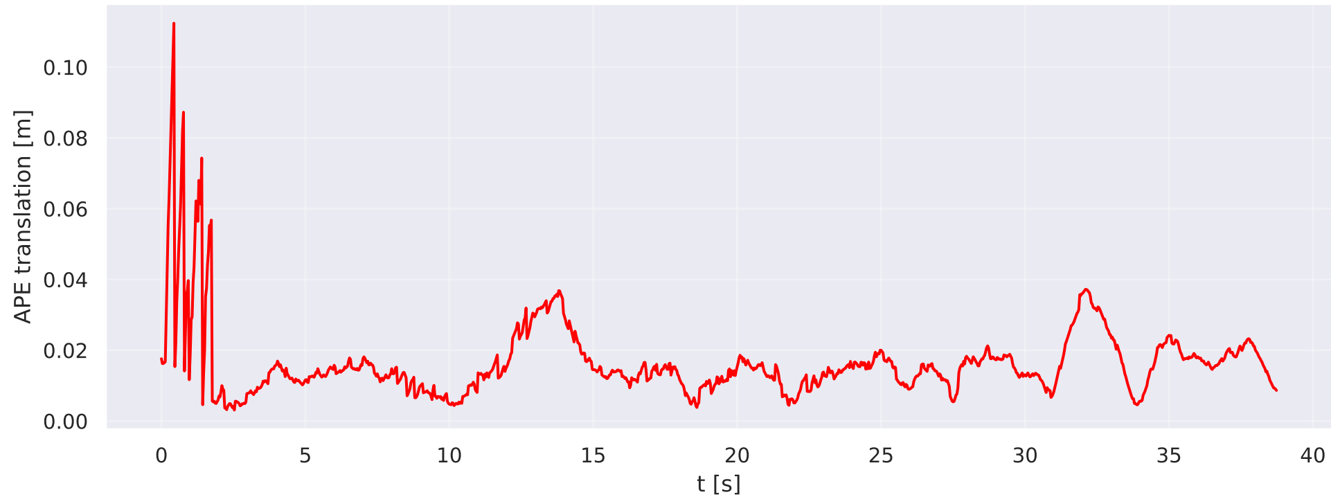
robot-normal DEIO(our run) — APE over time
