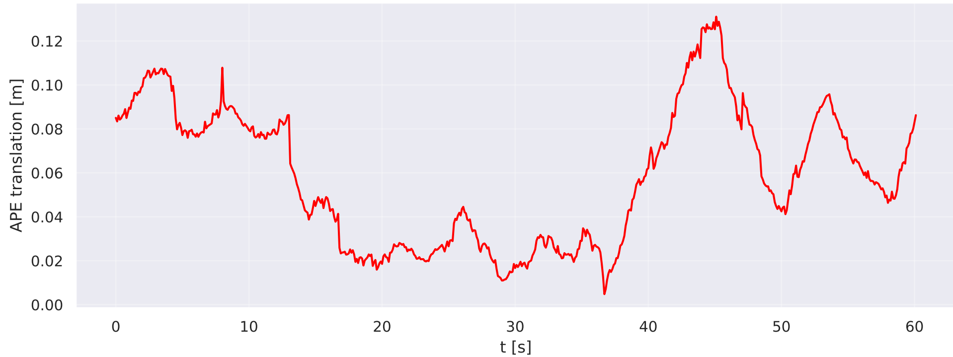
sdevo/vector/hdr-normal — APE over time
