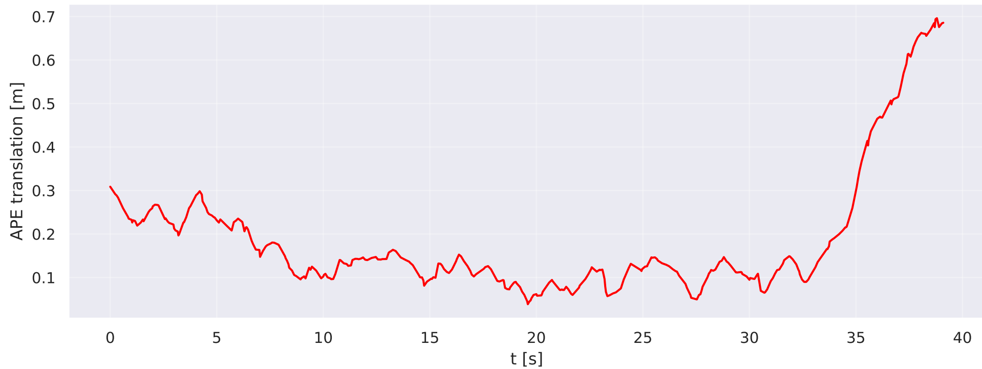
esvio/vector/hdr-fast — APE over time
