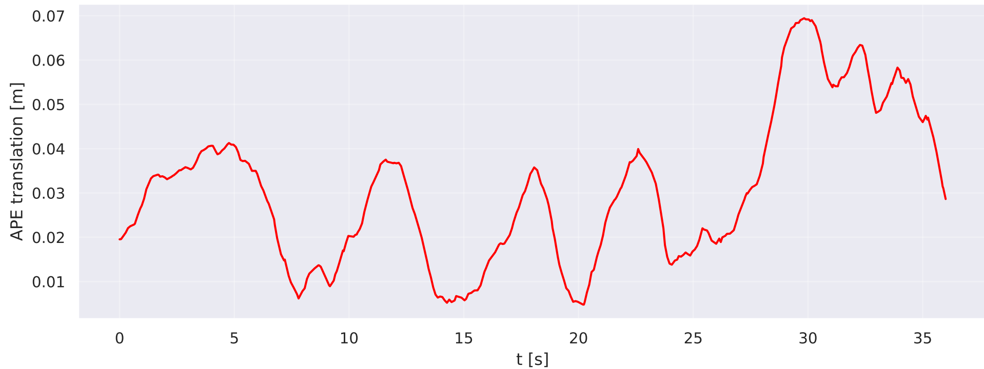
esvio/vector/robot-normal — APE over time
