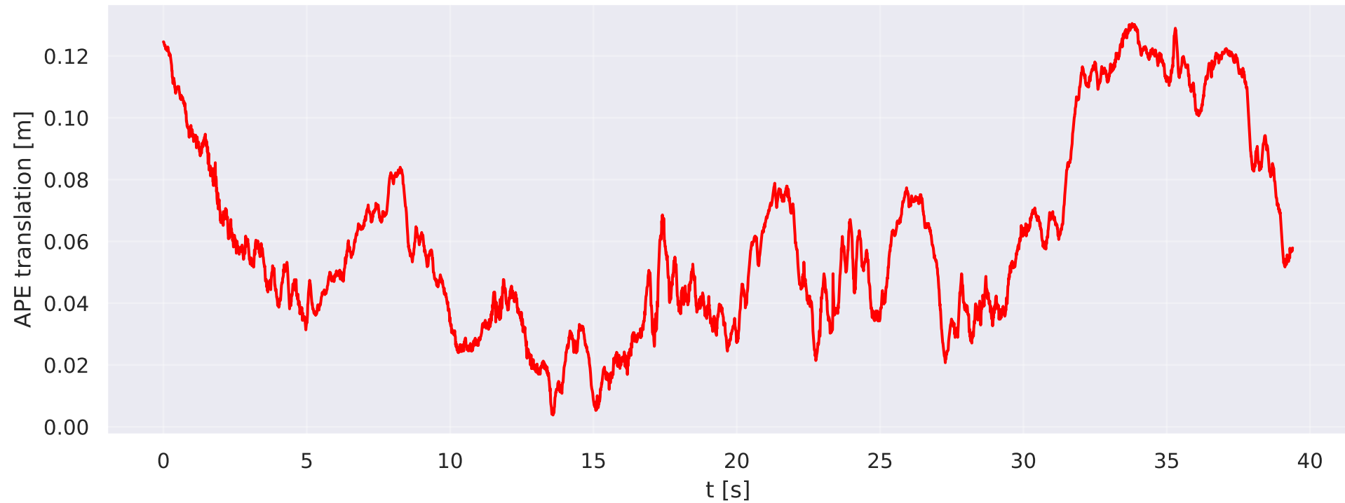
esvo2/vector/robot-normal — APE over time
