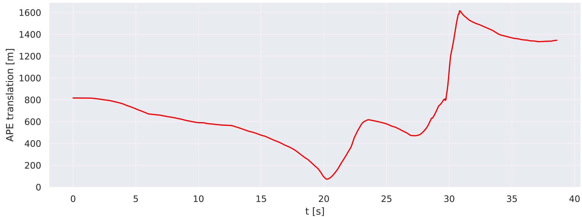
esvo2/vector/sofa-fast — APE over time
