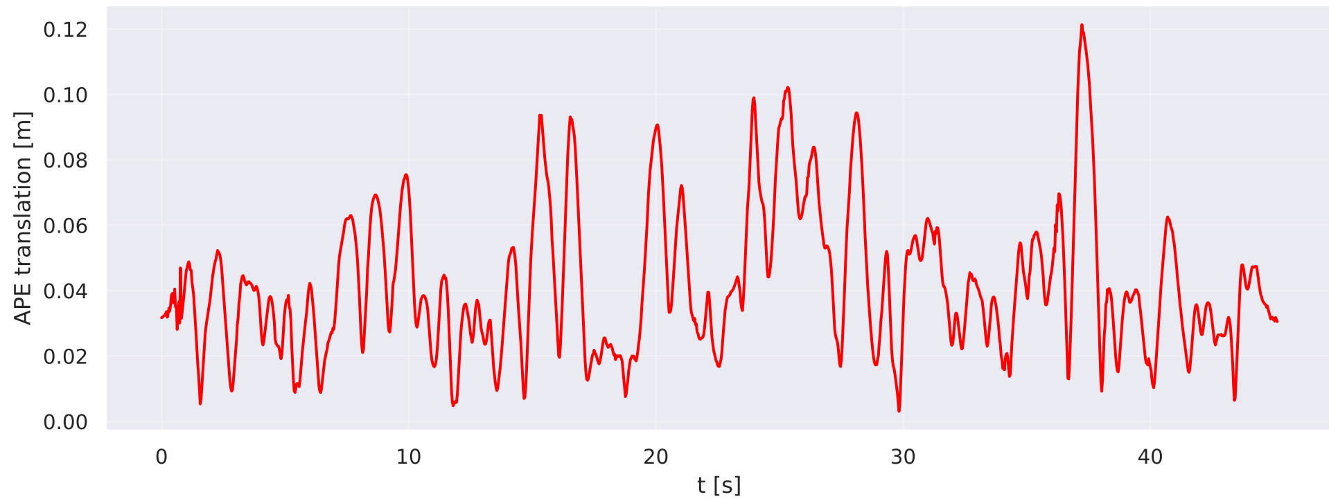
deio/vector/desk-fast — APE over time
