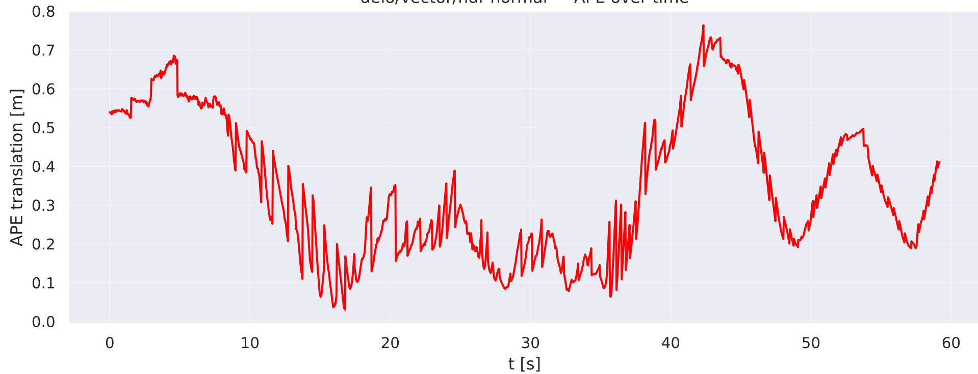
deio/vector/hdr-normal — APE over time
