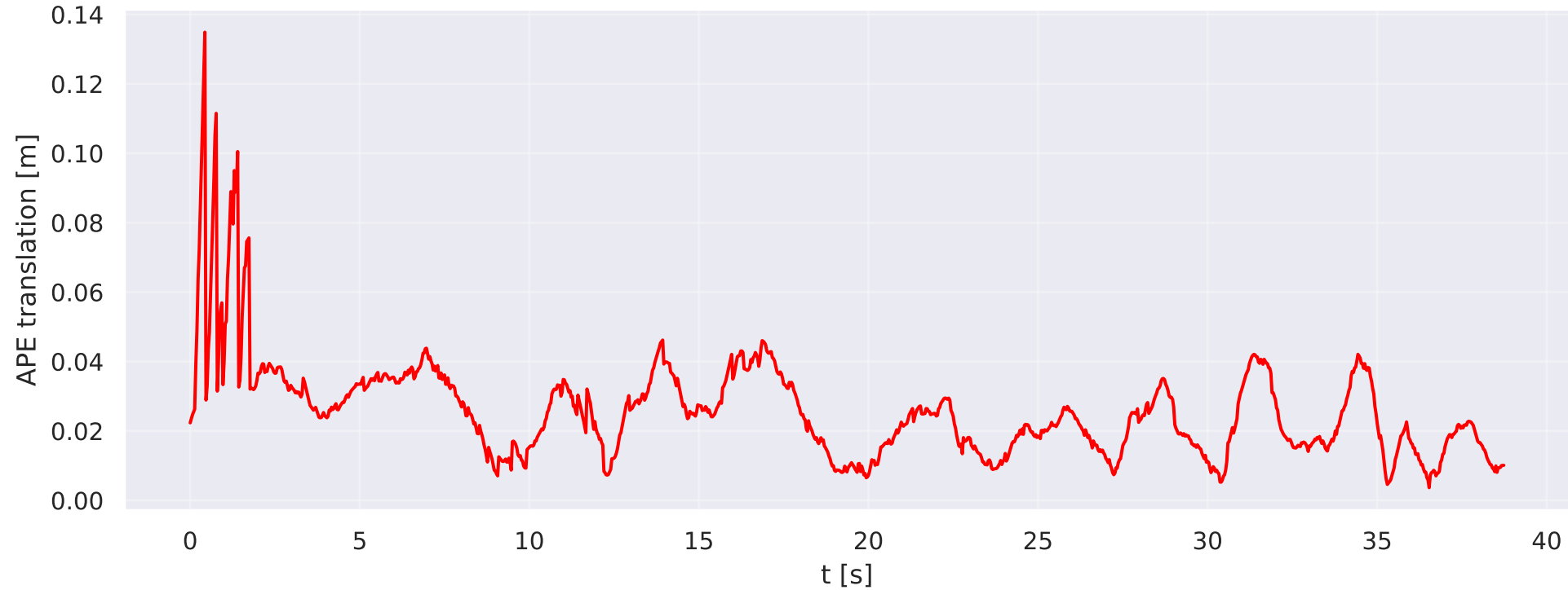
deio/vector/robot-normal — APE over time
