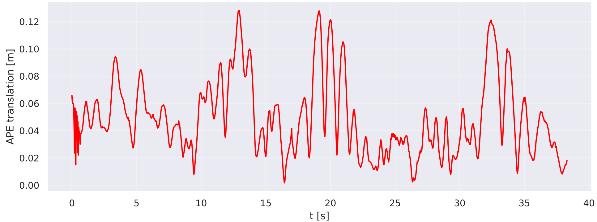
deio/vector/sofa-fast — APE over time
