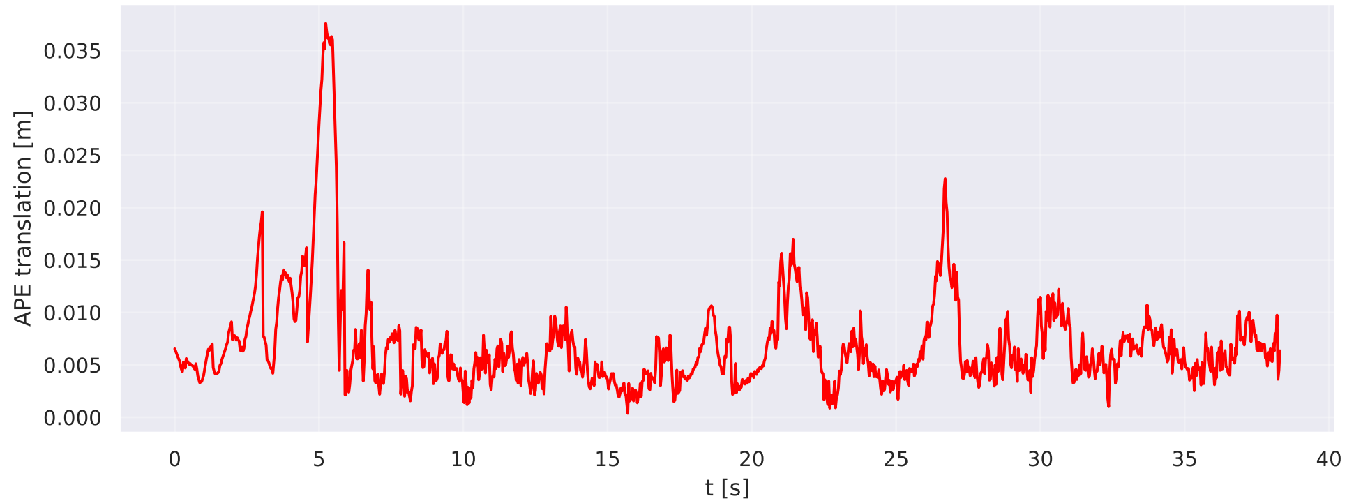
devo/vector/corner-slow — APE over time
