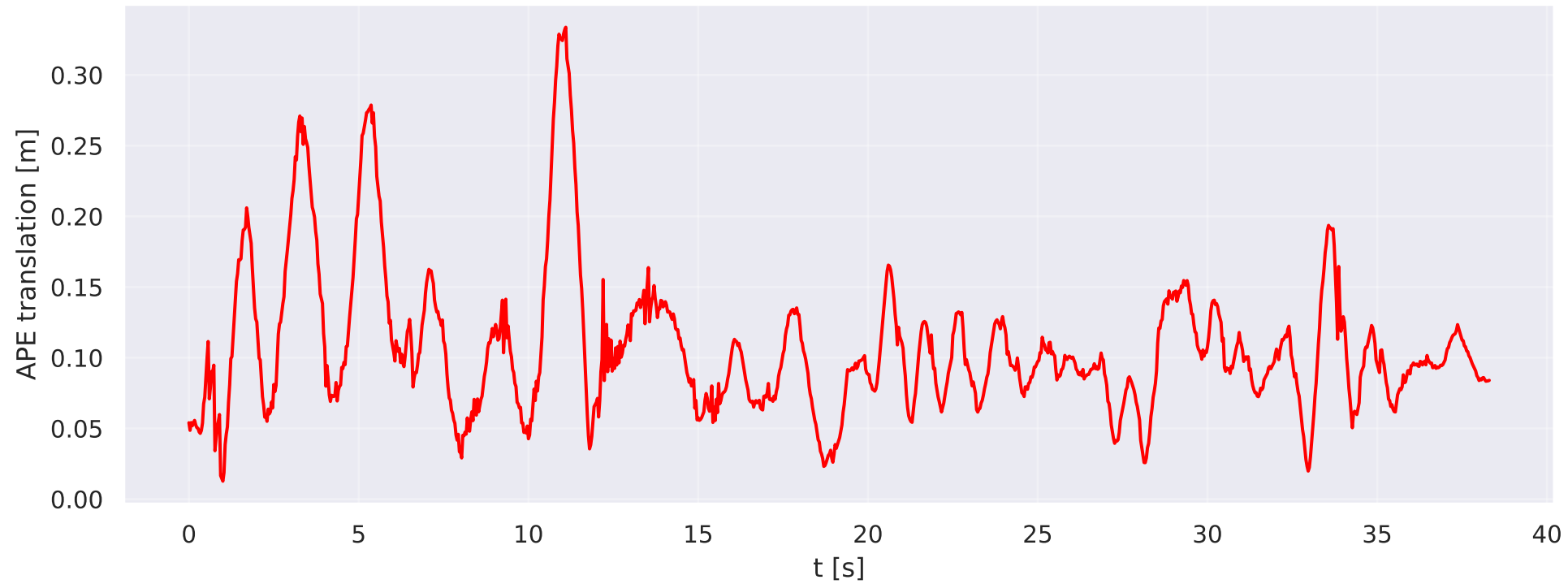
devo/vector/sofa-fast — APE over time
