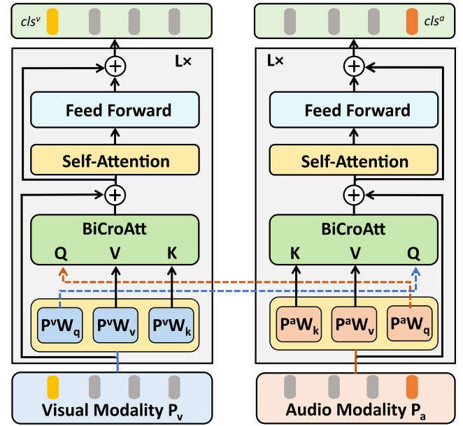
Fig. 4. The Multi-Modal Joint-Decoder (MMD). MMD is the modal fusion part of AVoid-DF. The input embedded patches of vision and sound will be fed through two parallel decoder channels. Each channel has a Bi-directional Cross-attention (BiCroAtt) block followed by self-attention and feed forward layers. BiCroAtt enables the information sharing between two modalities for joint learning.
