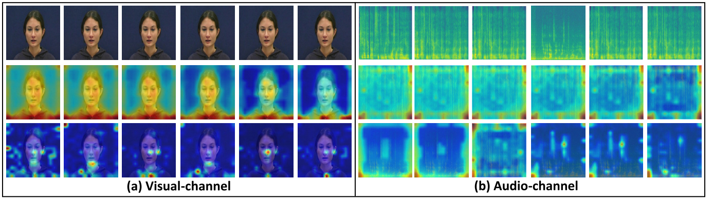
Fig. 6. The visualization result of uni-modal learning and multi-modal joint learning. Row 1 denotes the raw data inputs, which are sampled from our proposed dataset. Row 2 represents the distribution of attention values with uni-modal input. Apparently, deepfake forgeries are not well detected due to the double interference from background noise and non-forged areas. Row 3 is the distribution of attention values with the fusion of two modalities in our model. We can conclude that the audio-visual multi-modal help with locating forged area through a more refined local and global attention.
