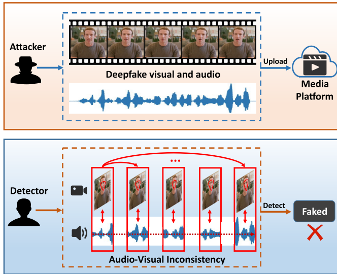
Fig. 1. The motivation for detecting deepfake with audio-visual. Attackers aim to generate forged videos with both visual and audio maliciously modified. The uploaded videos can pose a looming threat to everyone on the platform. Our method focuses on exploiting the audio-visual inconsistency among temporal and spatial information for multi-modal deepfake detection. The detector can effectively distinguish whether the media contains forged visual or audio to help against deepfake attacks.
