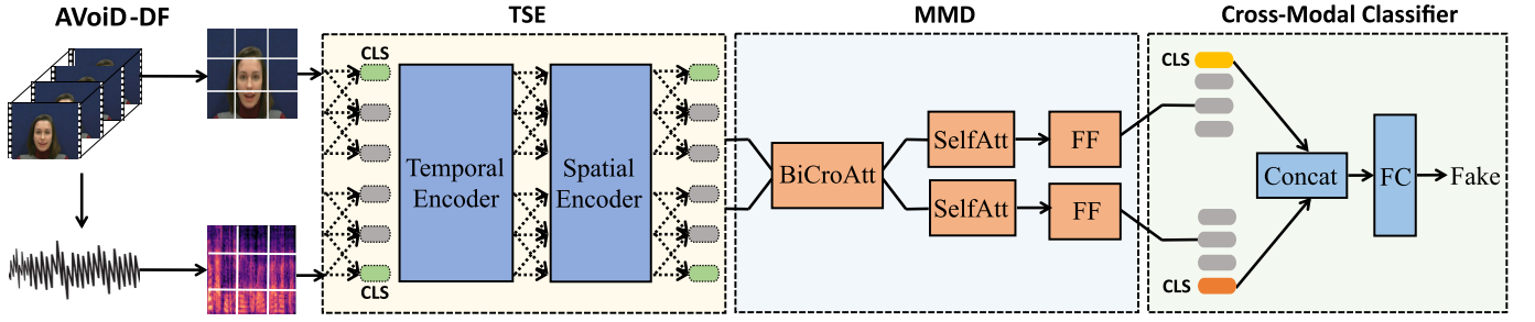
Fig. 2. Overview of our proposed AVoid-DF. In the entry flow, the input visual and audio are first sampled and sliced into patches through data pre-processing. After that, the audio-visual patches are fed into a two-stream Temporal-Spatial Encoder (TSE) to extract features and embed temporal-spatial information. In the fusion flow, Multi-Modal Joint-Decoder (MMD) reads the audio-visual features and fuses them for jointly learning inherent relationships. Finally, the classification tokens of two modalities are selected and concatenated. And the Cross-Modal Classifier together with loss function is exploited to limit the inter-class distance and detect deepfakes.
