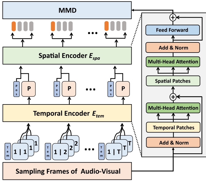
Fig. 3. The Temporal-Spatial Encoder (TSE). This module consists of two transformer encoders in series. The first temporal encoder models interactions between time steps of the same window and embeds temporal information. The second spatial encoder produces a latent representation of spatial characteristics per time-index. It thus corresponds to a late fusion of temporal-spatial information. Then the embedded features of two modalities will be output in parallel and sent to the MMD for multi-modal fusion.
