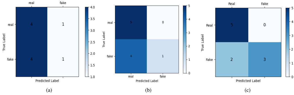
Fig. 2: Confusion matrix (a) CNN with GRU (b)XceptionNet with GRU (c) LSTM with RestNext50
