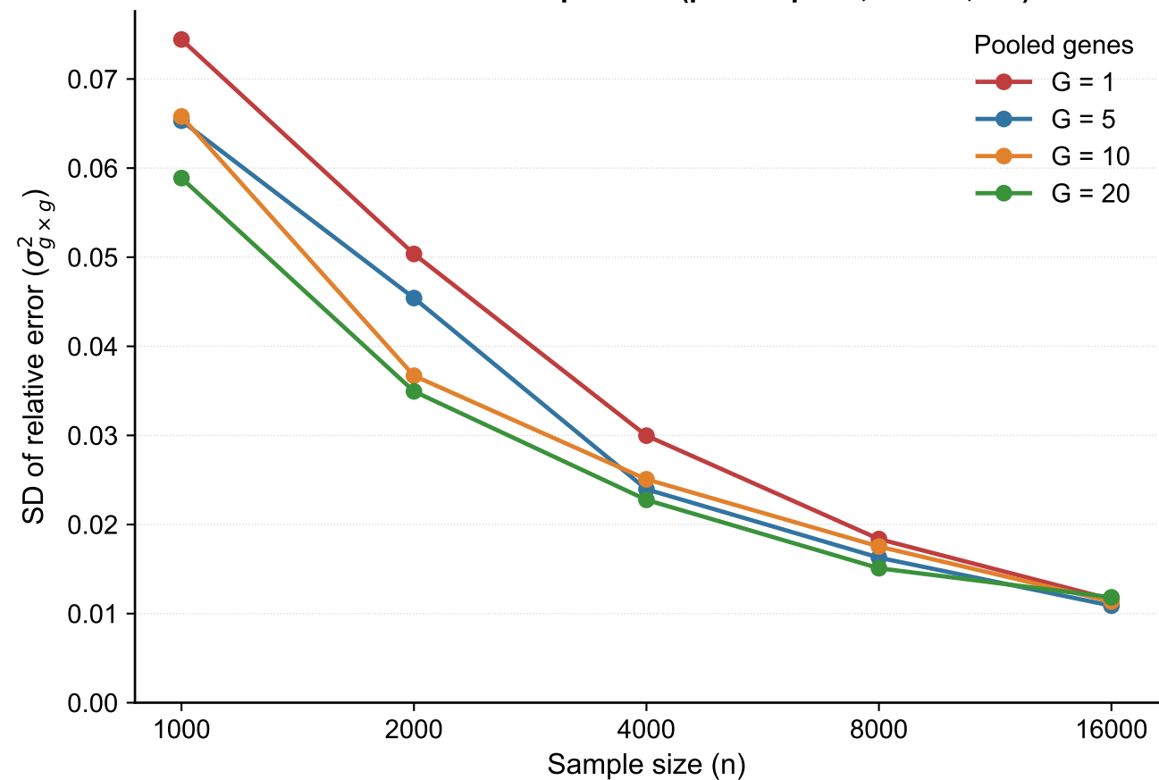
Estimation SD vs sample size (pooled preW, m = 10,000)
