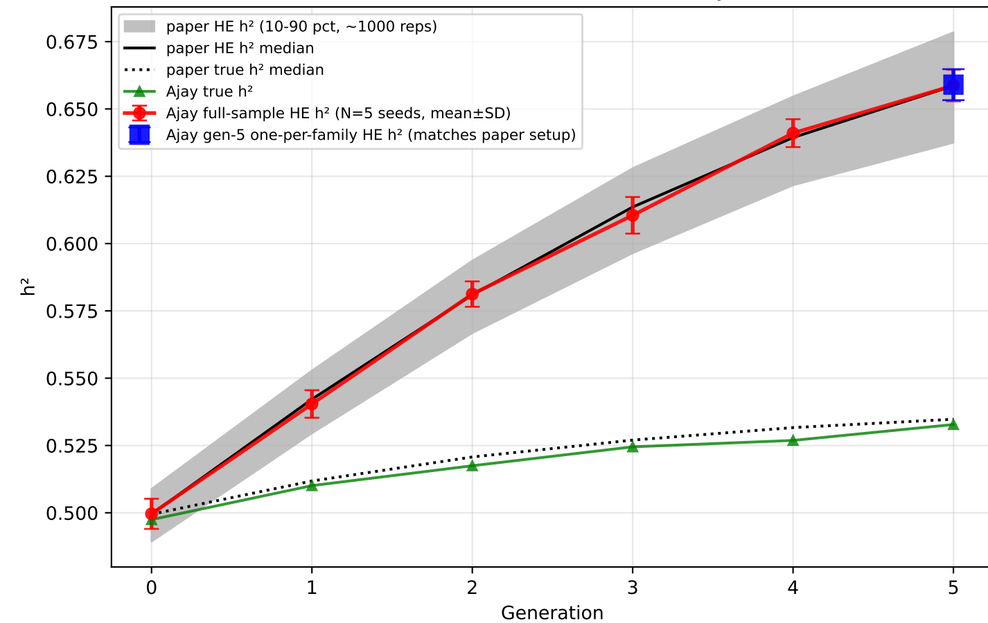
5xAM: HE-estimated heritability
