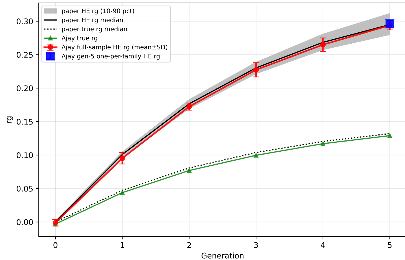
5xAM: HE-estimated genetic correlation
