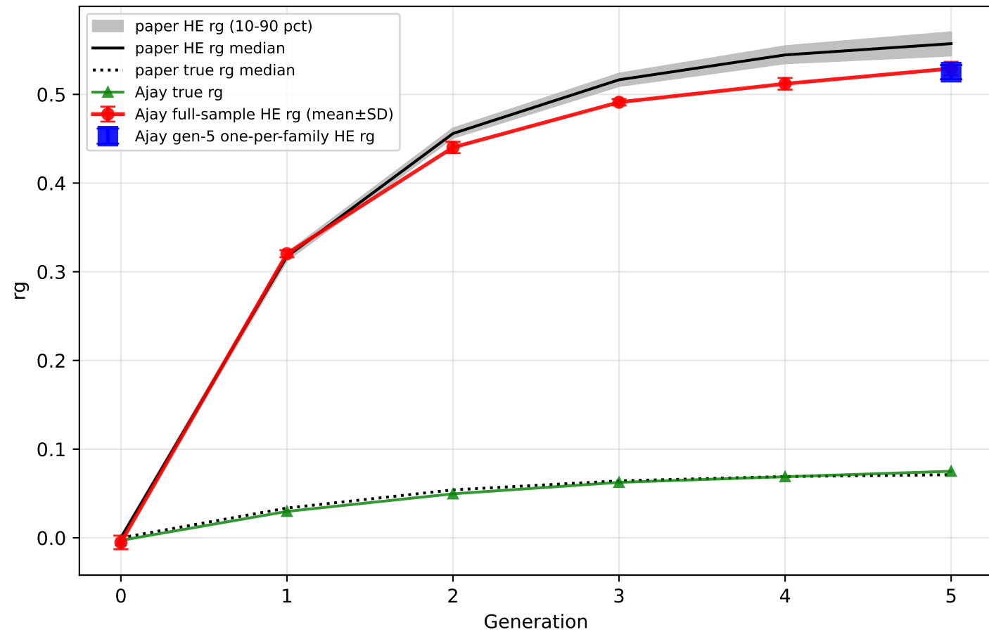
5xAM+VT: HE-estimated genetic correlation
