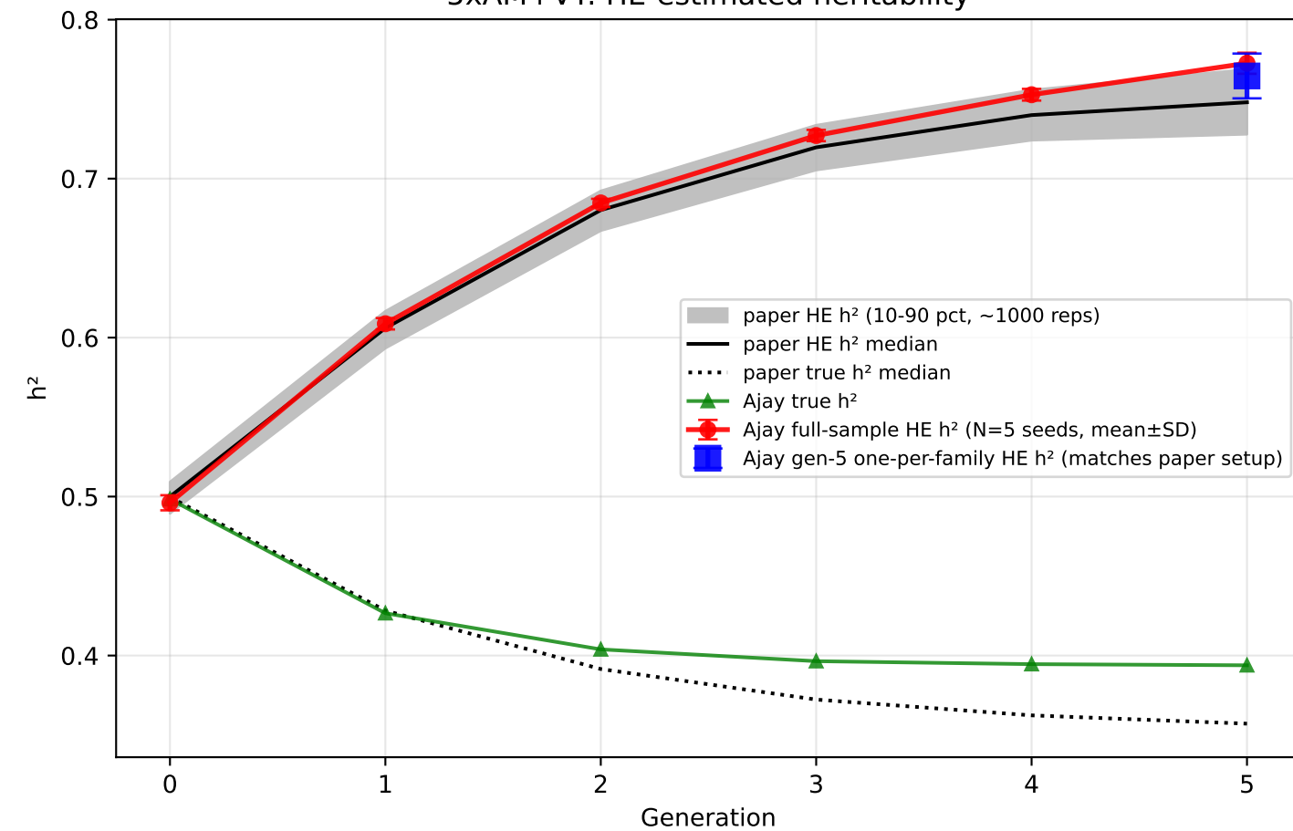
5xAM+VT: HE-estimated heritability
