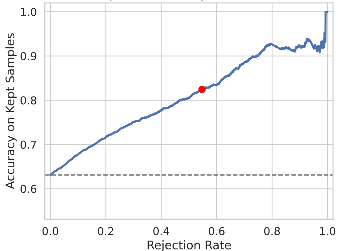
Rejection Accuracy Curve (RAC)
