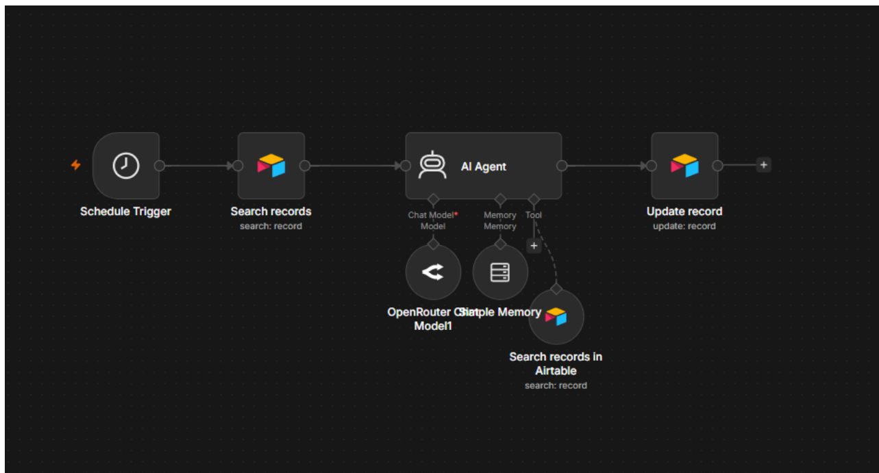
Figura 2. Workflow principal en n8n: Schedule Trigger, Airtable, AI Agent, OpenRouter, Memory, Tool de stock y Update record.
