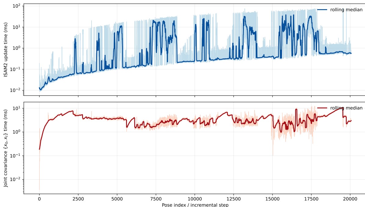
Figure 16: Sequential iSAM2 timing on w20000 with the pairwise joint covariance query \{x_0, x_t\} after every update. The light traces show raw per-step timings, while the dark curves show a rolling median over 100 steps. The update cost spikes when relinearization and re-elimination affect larger portions of the tree, whereas the covariance query remains in a much tighter few-millisecond band once the path to the current pose becomes long.
