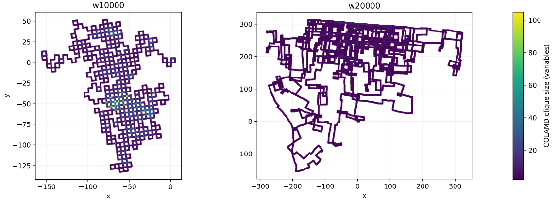
Figure 15: Final optimized trajectories for w10000 and w20000 , colored by the size of the COLAMD Bayes-tree clique containing each pose. The two panels share one color scale. Several neighborhoods in w10000 pass through much larger cliques, whereas w20000 stays dominated by smaller cliques even though the trajectory is longer.
