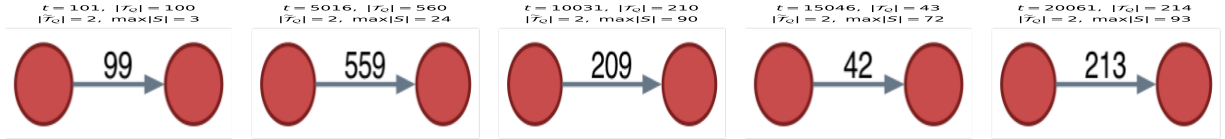
Figure 17: Five compressed-support snapshots for the pair query \{x_0, x_t\} during the sequential w20000 run. Each edge represents one shortcut-compressed chain of support cliques, and the edge label gives the number of raw support cliques absorbed into that shortcut segment.
