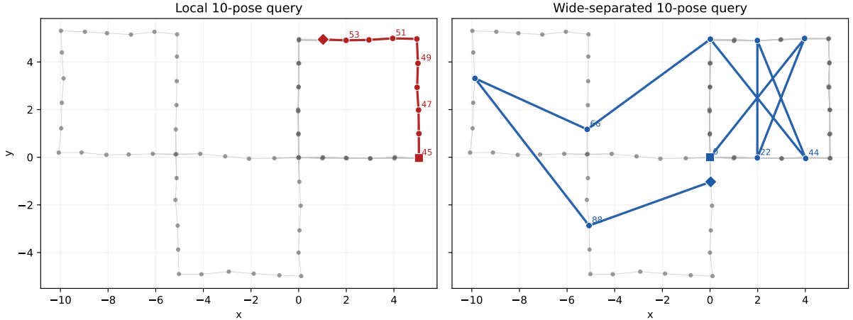
Figure 10: The w100 pose graph makes the benchmark query families concrete. The left panel highlights a contiguous 10-pose local window, while the right panel highlights a 10-pose wide-separated query spread across the map. These two query shapes induce very different Steiner supports and therefore very different covariance-query costs.
