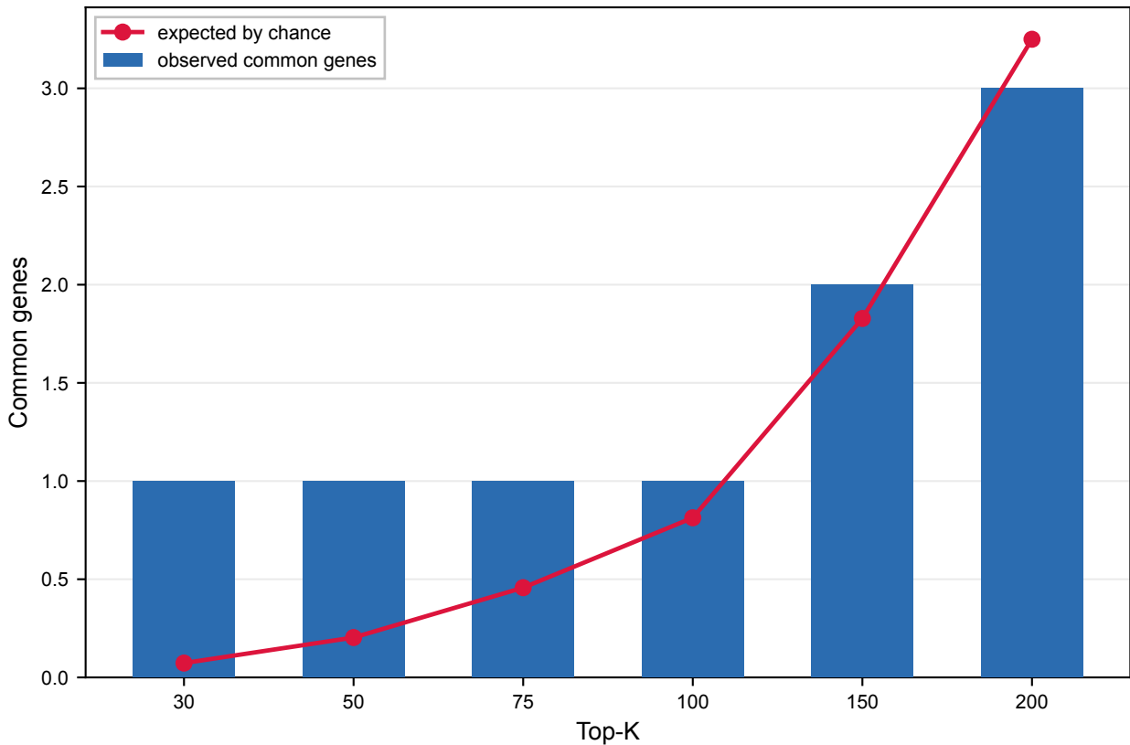
Severity top-K vs Warning sign top-K overlap
