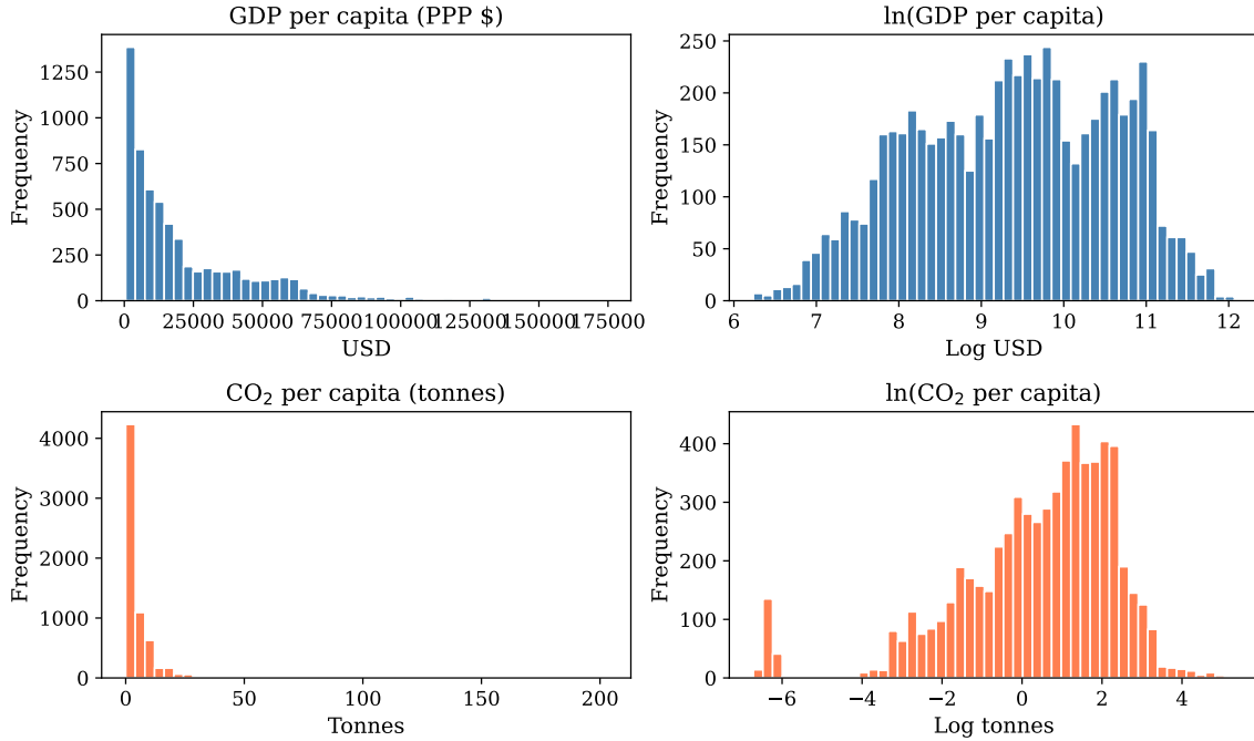
Figure 1: Distribution of GDP and CO 2 per capita in levels (left) and logs (right). The log transform removes the heavy right skew and produces approximately symmetric distributions.
