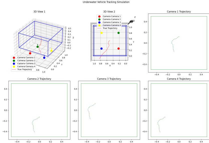
Figure 3: 3D simulation environment with virtual camera array and AUV trajectories.
