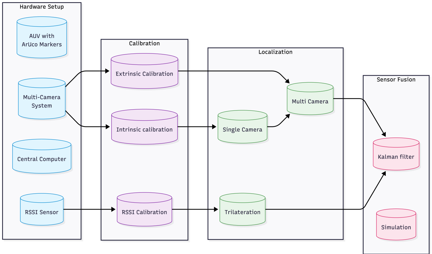
Figure 2: MASEP localization system block diagram.
