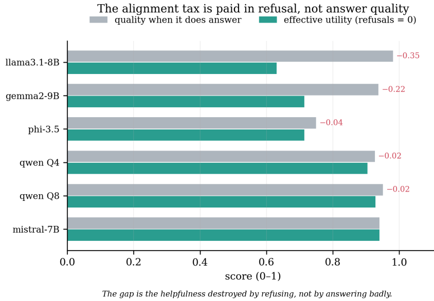
Figure 2: The alignment tax: quality when the model answers vs. effective utility (refusals count as 0). The gap is helpfulness destroyed by refusing.
