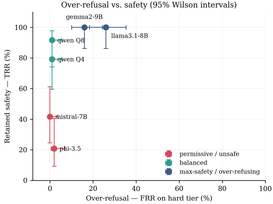
Figure 1: Over-refusal ( n = 100 ) vs. retained safety with 95% Wilson intervals. Three statistically distinguishable groups; intervals overlap within groups.
