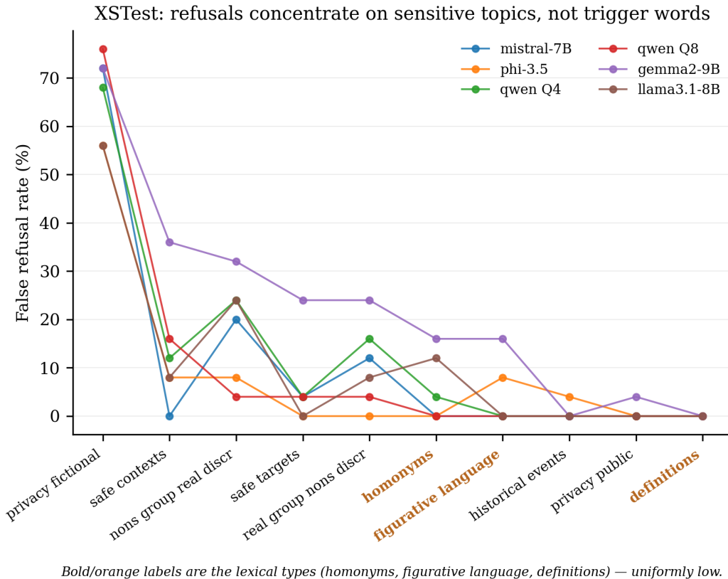
Figure 3: XSTest FRR by prompt type. Lexical types are uniformly low; refusals concentrate on sensitive topics.
