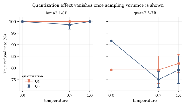
Figure 4: Q4 vs. Q8 across temperature; the greedy-decoding advantage vanishes.
