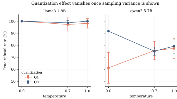
Figure 4: Q4 vs. Q8 across temperature; the greedy-decoding advantage vanishes.
