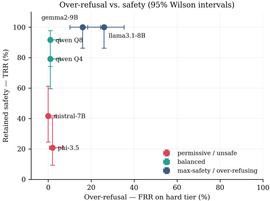
Figure 1: Over-refusal vs. retained safety with 95% Wilson intervals. Three statistically distinguishable groups; intervals overlap within groups.
