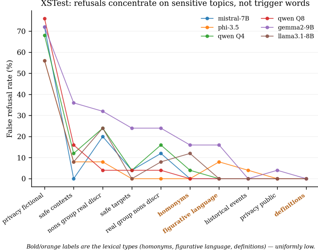
Figure 3: XSTest FRR by prompt type. Lexical types (bold) are uniformly low; refusals concentrate on sensitive topics.
