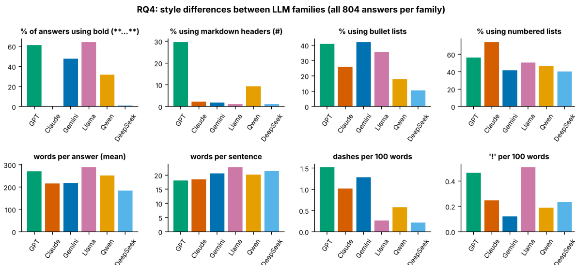
Figure 2. Style differences between the LLMs. Top row: % of answers that use each kind of formatting at least once. Bottom row: averages.
