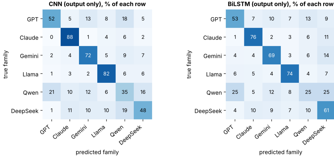
Figure 1. Confusion matrices on the test set (3 seeds together). Each row is the true LLM and shows where its answers went (% of the row). The diagonal is the share of that LLM’s answers that were labeled correctly.
