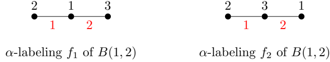
Figure 6: Two \alpha -labelings of B(1, 2)
