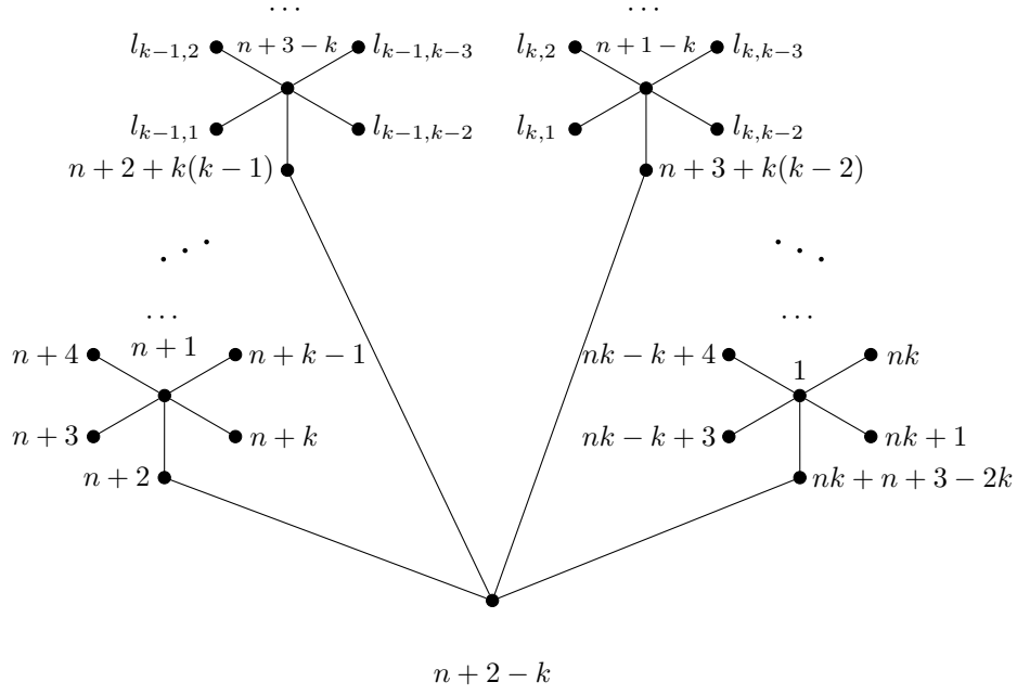
Figure 10: The labeling f of the B(n, k) tree
