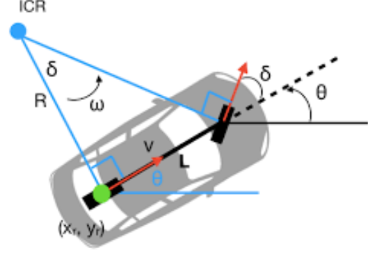
Figure 3: Schematic of bicycle model.
