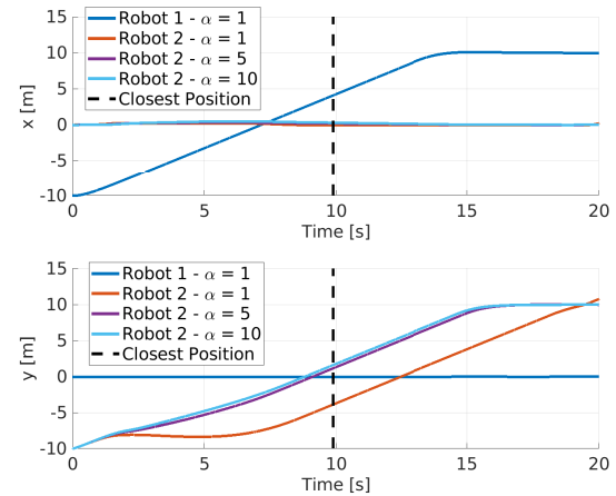
Figure 6: Position of both robots. Robot 1 runs nominal controller only, and Robot 2 uses CBF to avoid collision.
