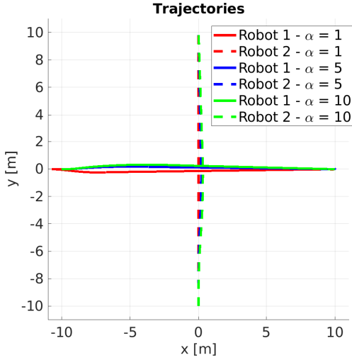
Figure 4: Trajectories of robots with unicycle kinematics for different \alpha values.
