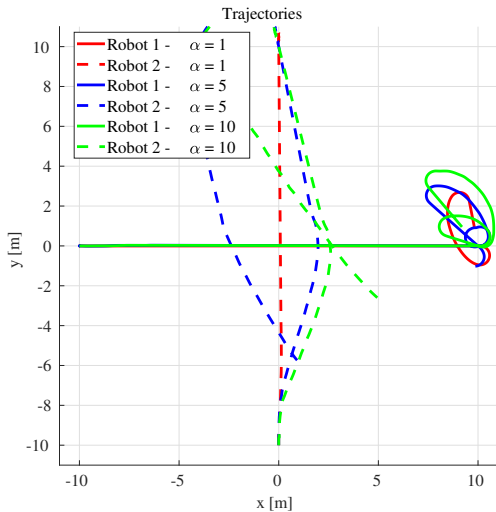
Figure 7: Trajectory of robots with bicycle kinematics for different \alpha values.
