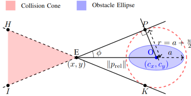
Fig. 1: Construction of collision cone for an elliptical obstacle considering the ego vehicle's dimensions (width w ).
