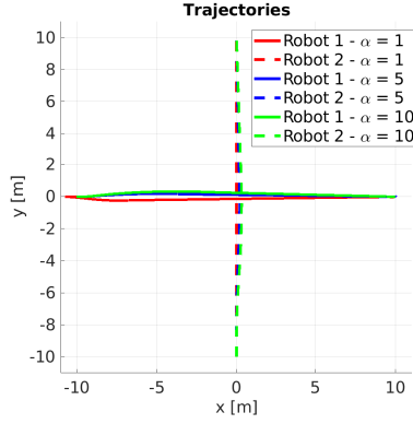
Fig. 3: Trajectories of robots with unicycle kinematics for different \alpha values.
