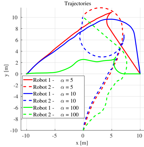
Fig. 6: Trajectory of robots with bicycle kinematics for different \alpha values.
