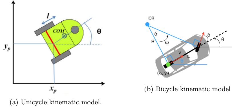
Fig. 2: Motion models schematic view.
