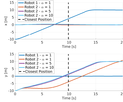
Fig. 5: Position of both robots. Robot 1 runs nominal controller only, and Robot 2 uses CBF to avoid collision.
