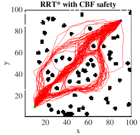
Fig. 4. Exemplary results of 100 different runs of CBF-RRT* algorithm for Scenario I - for 0.5 \frac{m}{s} target speed.
