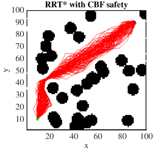
Fig. 7. Exemplary 100 different runs of CBF-RRT* algorithm for Scenario II - for 2 \frac{m}{s} target speed.
