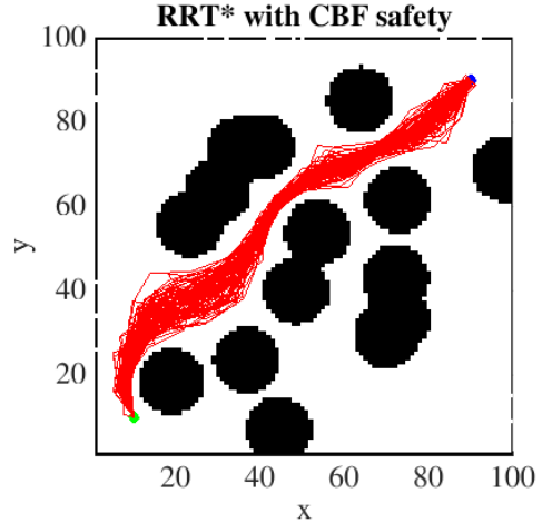
Fig. 11. Exemplary 100 different runs of CBF-RRT* algorithm for Scenario III - for 2 \frac{m}{s} target speed.
