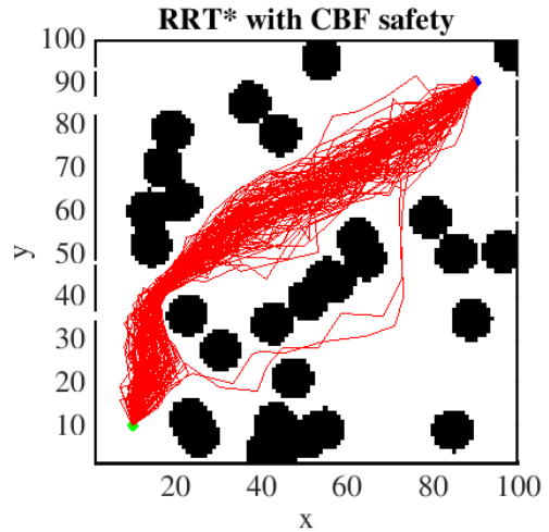
Fig. 8. Exemplary 100 different runs of CBF-RRT* algorithm for Scenario II - for 0.5 \frac{m}{s} target speed.
