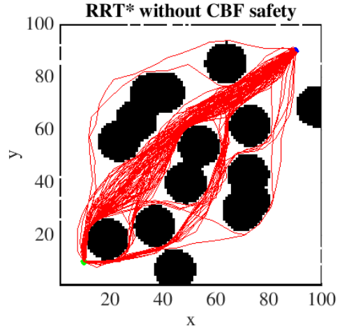
Fig. 10. Exemplary 100 different runs of standard RRT* algorithm for Scenario III.
