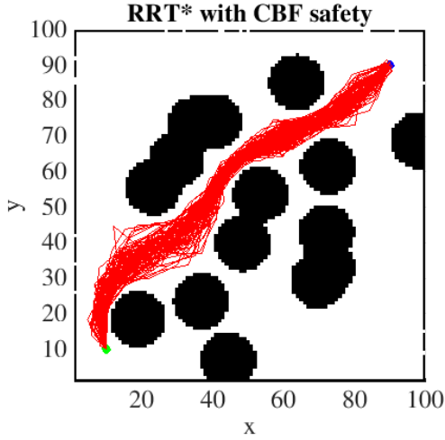
Fig. 12. Exemplary 100 different runs of CBF-RRT* algorithm for Scenario III - for 0.5 \frac{m}{s} target speed.
