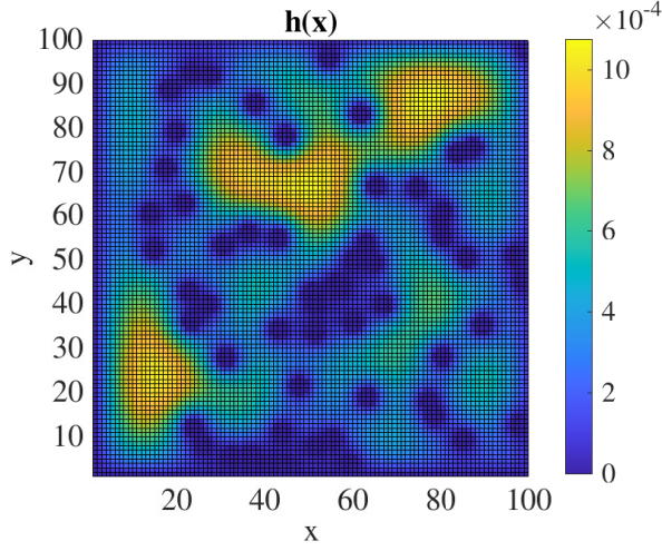
Fig. 1. Control barrier function for Scenario I.
