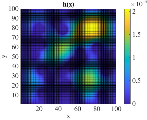
Fig. 5. Control barrier function for Scenario II.
