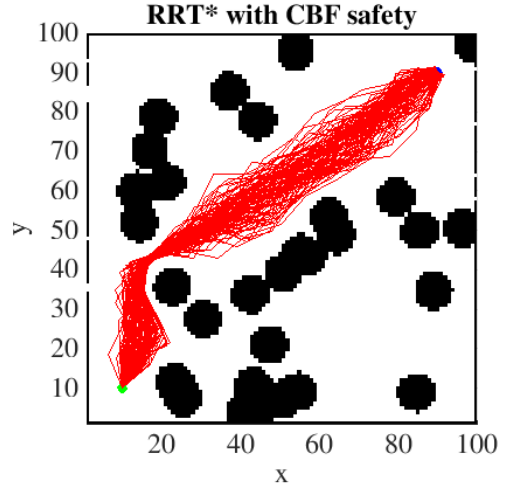
Fig. 6. Exemplary 100 different runs of CBF-RRT* algorithm.
