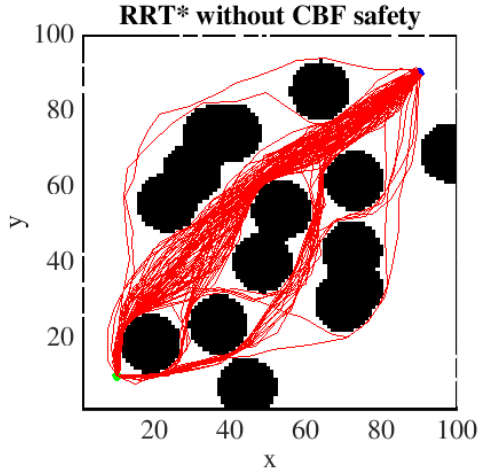
Fig. 8. Exemplary 100 different runs of standard RRT* algorithm.
