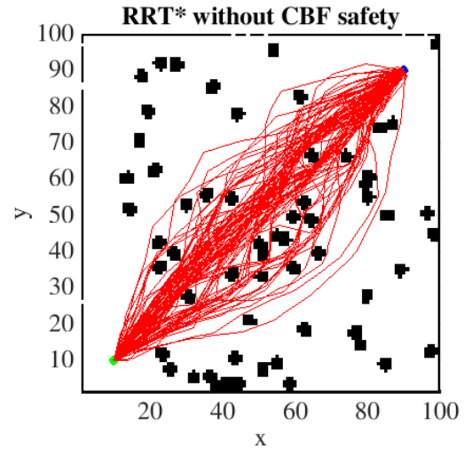
Fig. 2. Exemplary results of 100 different runs of standard RRT* algorithm.
