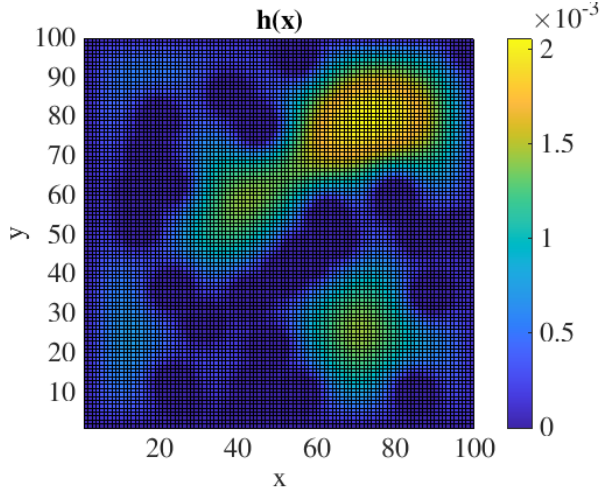
Fig. 4. Control barrier function for scenario II.
