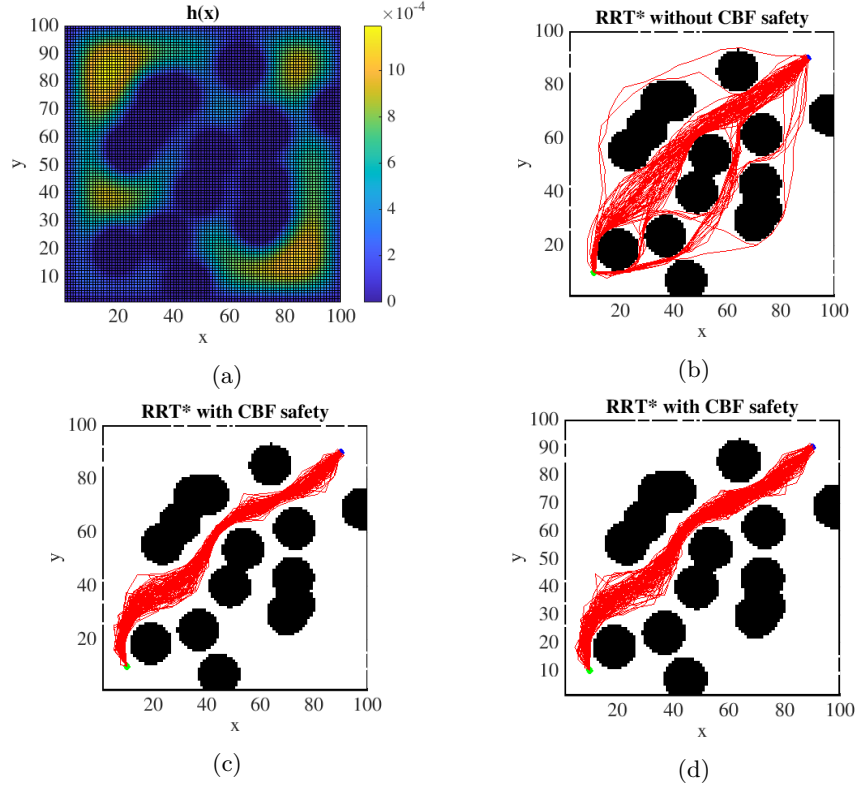
Fig. 3: Example results of 100 different runs for Scenario III: (a) Control barrier function, (b) standard RRT*, (c) CBF-RRT* for 2 \frac{m}{s} target speed, (d) CBF-RRT* for 0.5 \frac{m}{s} target speed.
