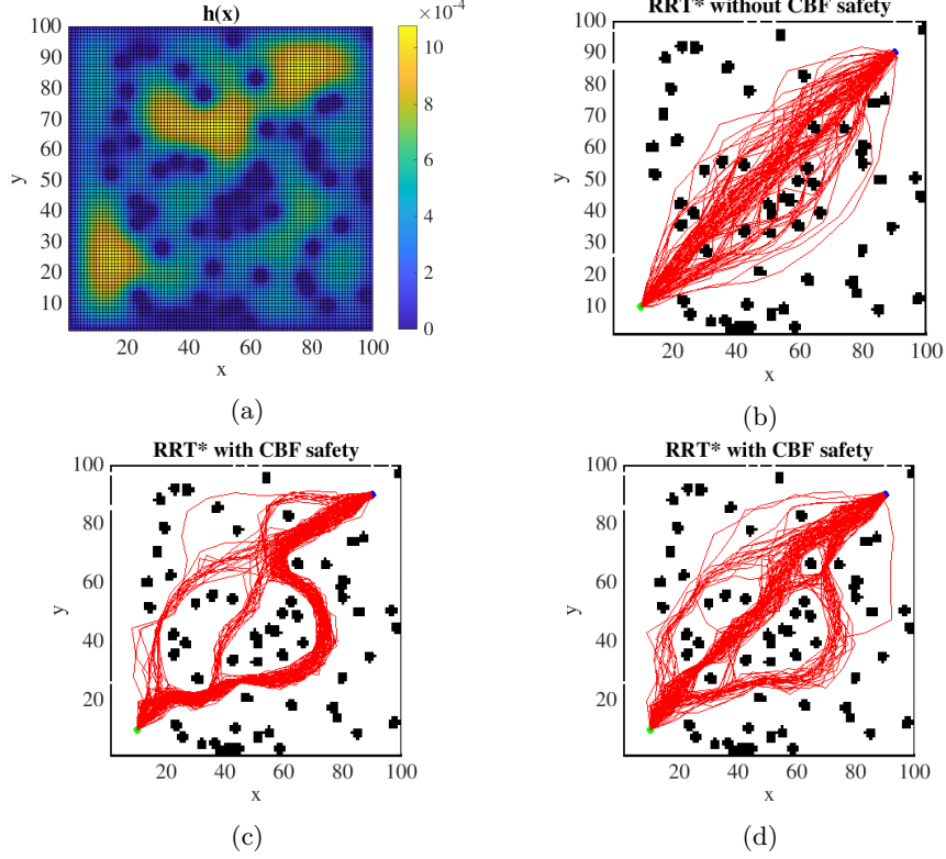
Fig. 1: Example results of 100 different runs for Scenario I: (a) Control barrier function, (b) standard RRT*, (c) CBF-RRT* for 2 \frac{m}{s} target speed, (d) CBF-RRT* for 0.5 \frac{m}{s} target speed.
