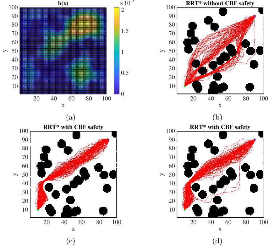
Fig. 2: Example results of 100 different runs for Scenario II: (a) Control barrier function, (b) standard RRT*, (c) CBF-RRT* for 2 \frac{m}{s} target speed, (d) CBF-RRT* for 0.5 \frac{m}{s} target speed.
