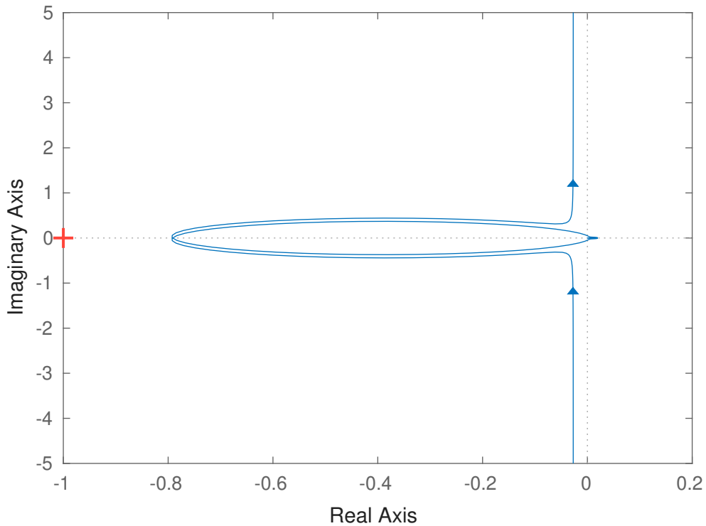
Nyquist Diagram
