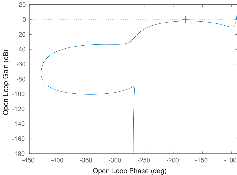
Nichols Chart
