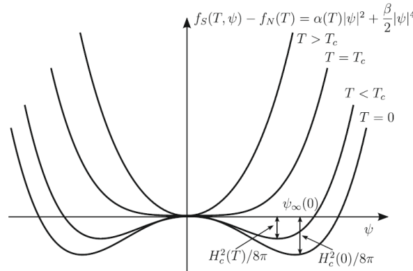
Figure 13: Temperature dependence of the Ginzburg-Landau free energy density as a function of the order parameter, showing the transition from a single minimum at \psi = 0 to a degenerate set of minima at finite |\psi| .
