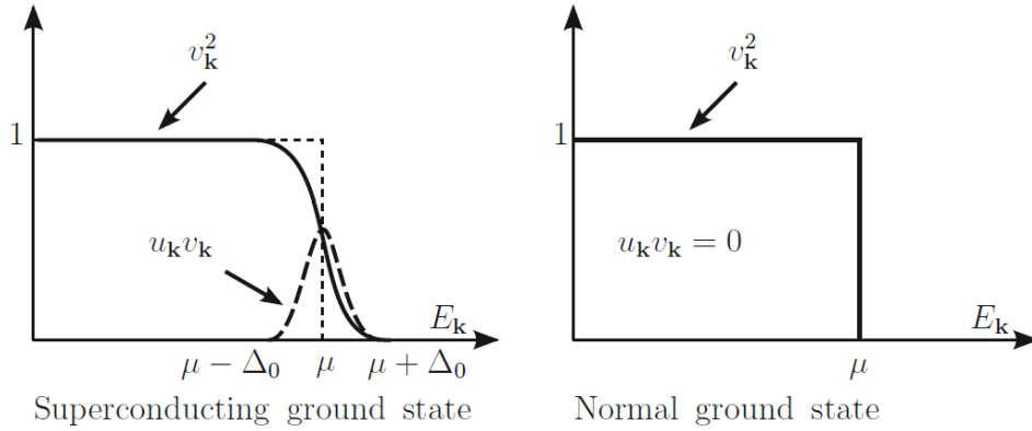
Figure 7: Schematic behavior of the quantities v_{\vec{k}}^2 and u_{\vec{k}}v_{\vec{k}} for both the superconducting and normal ground states. In the superconductor, the distribution v_{\vec{k}}^2 is smeared over an energy range determined by the gap \Delta_0 around the chemical potential \mu .
