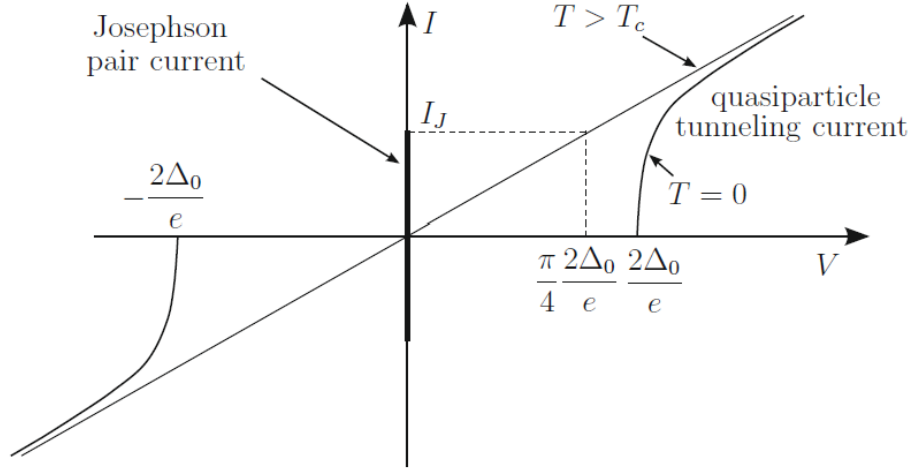
Figure 16: Schematic representation of the I-V characteristics for an SIS junction at T = 0 demonstrating the Josephson effect. The vertical line at V = 0 indicates the dc supercurrent up to I_J , while the region V > \frac{2\Delta_0}{e} shows the onset of quasiparticle tunneling.
