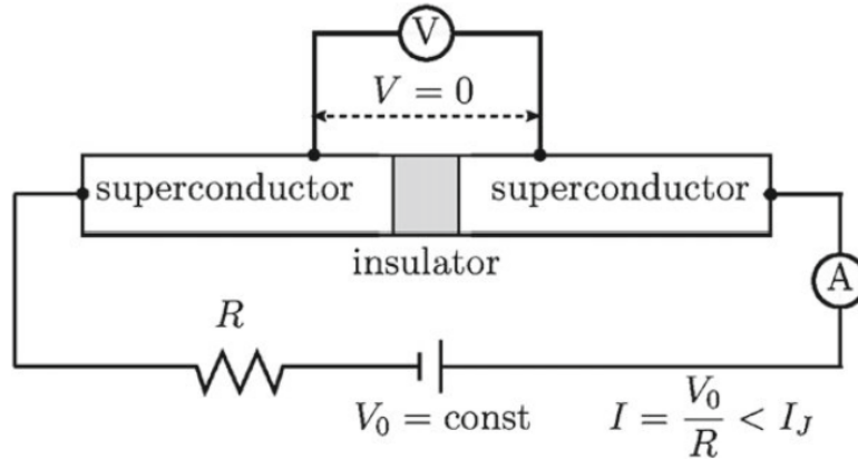
Figure 18: Schematic illustration of the dc Josephson circuit. A direct supercurrent flows through the insulating barrier, sustained by the phase coherence of the Cooper pair condensates.
